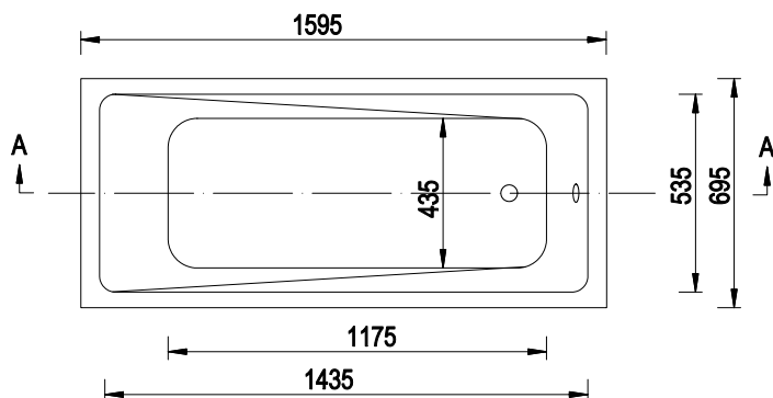
ELLEN SLIM 160x70 cm (EMPORIA-BS-WAM160)
