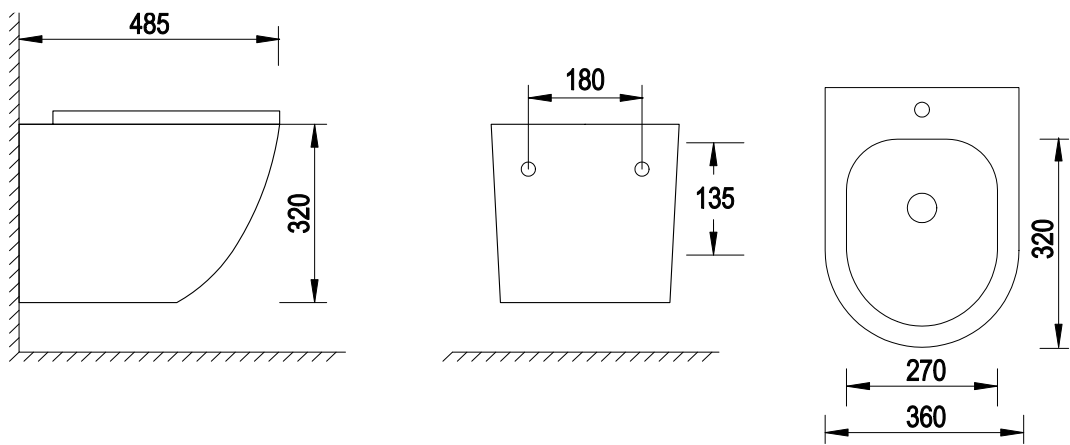
NOX 1.0 48,5x36x32 cm (EMPORIA-B0114)
