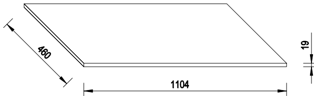
TOP 110,4x46x1,9 cm (EMPORIA-TOP-WHITE-1104 | EMPORIA-TOP-BLACK-1104)
