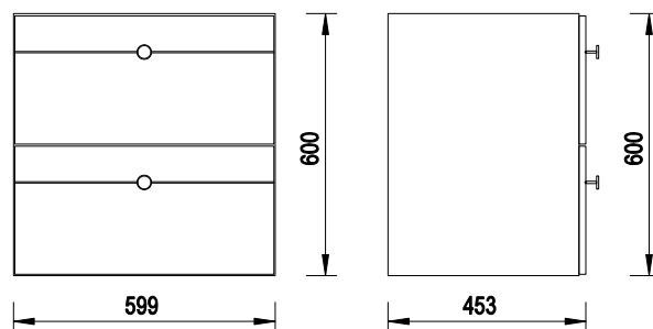
LOOP 60 59,9x45,3x60 cm (EMPORIA-001-D-06025)
