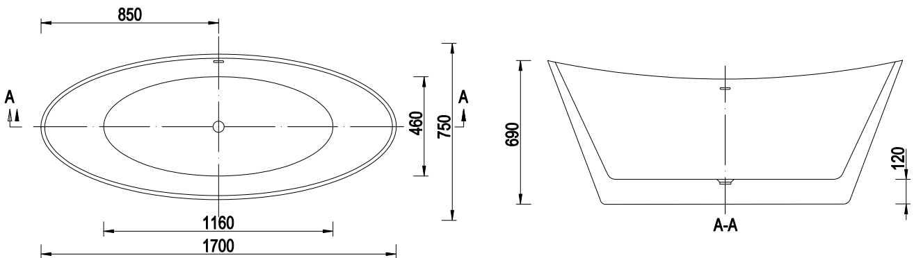
MONYA NEW 170x75x69 cm (EMPORIA-WS208P-NEW)
