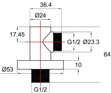
EMPORIA-04085 Built-In handshower
