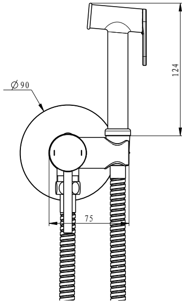
EMPORIA-03021 Concealed wall bidet
