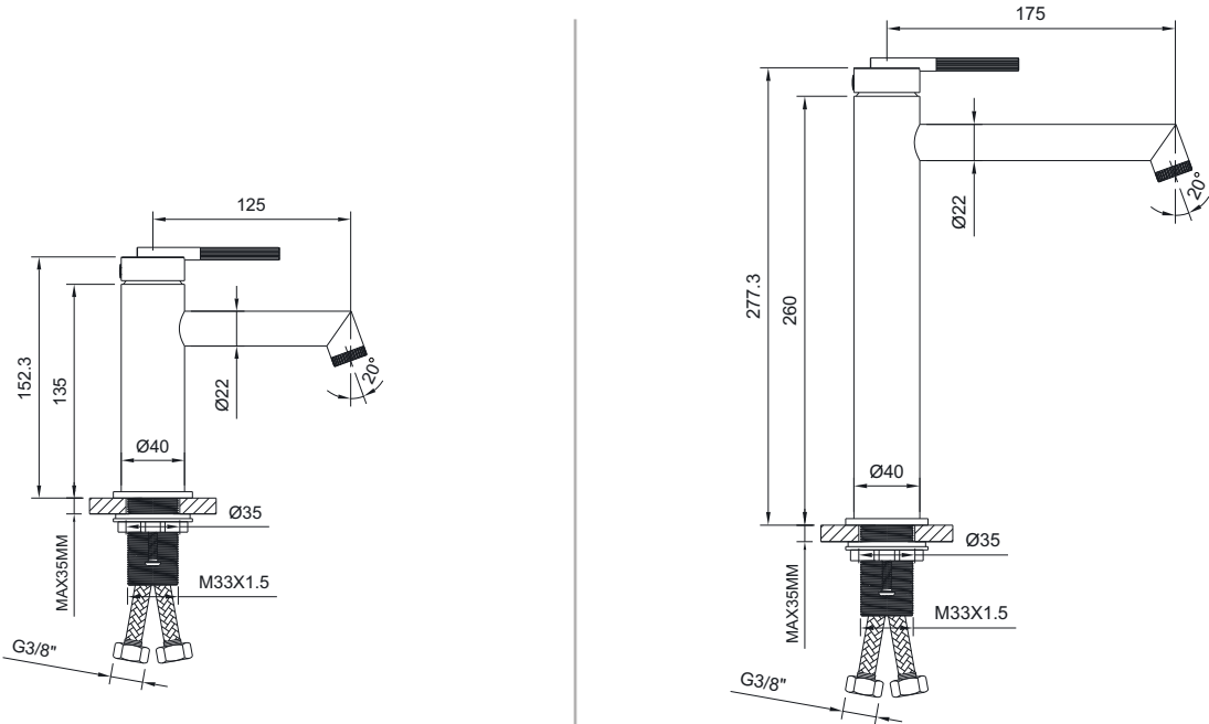
EMPORIA-01010 Basin mixer
