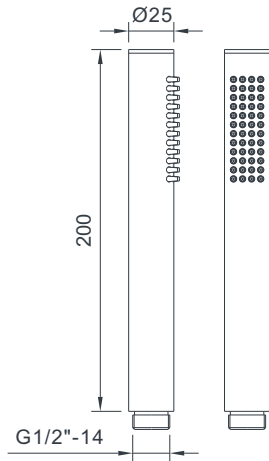
EMPORIA-040710 Shower hand
