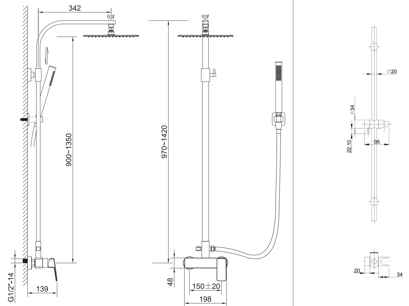
EMPORIA-020110 Rainshower mixer 2-function
