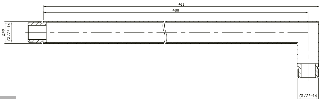
EMPORIA-04050 Shower arm
