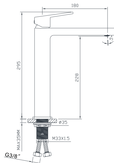
EMPORIA-02011 Basin mixer
