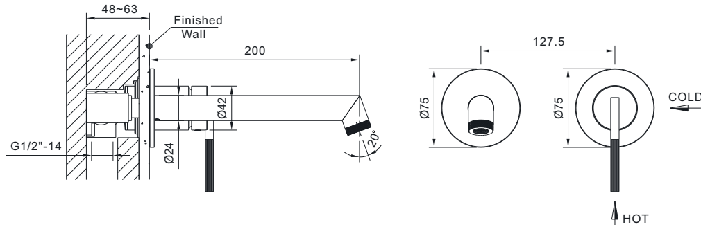
EMPORIA-01012 Concealed basin
