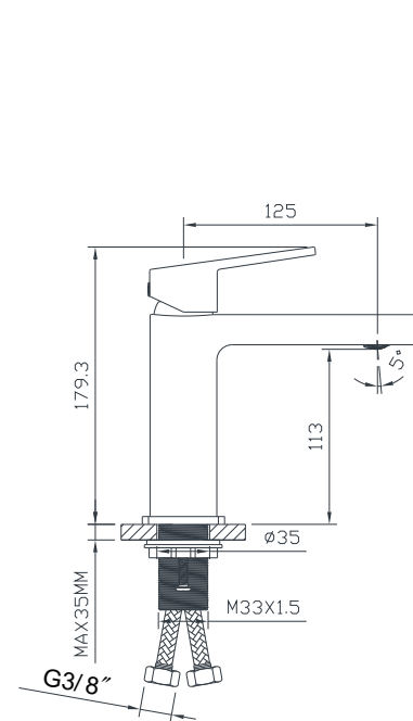
EMPORIA-02010 Basin mixer
