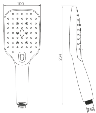
EMPORIA-040732 Shower hand
