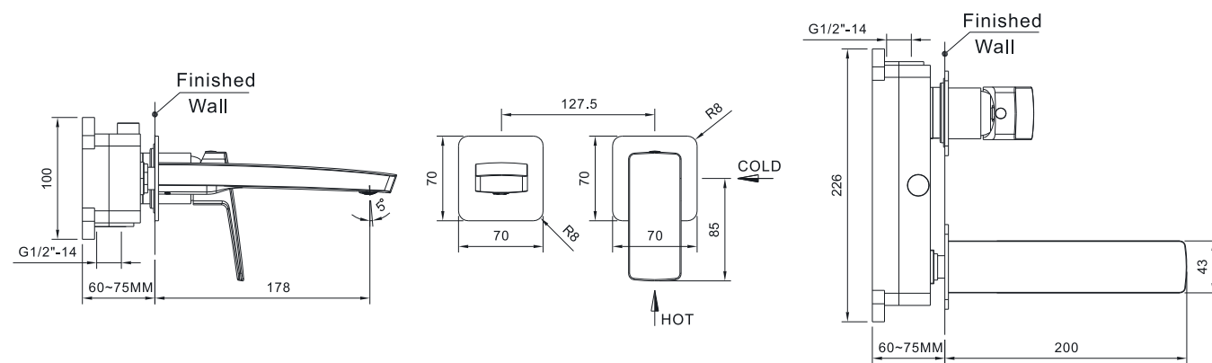
EMPORIA-02012 Concealed basin mixer
