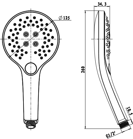
EMPORIA-040731 Shower hand
