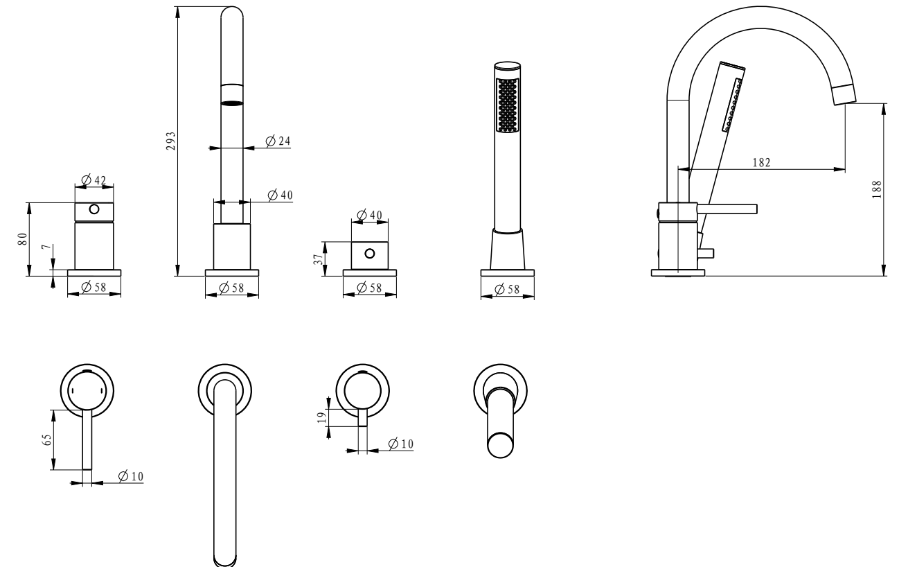
EMPORIA-03033 Bath mixer
