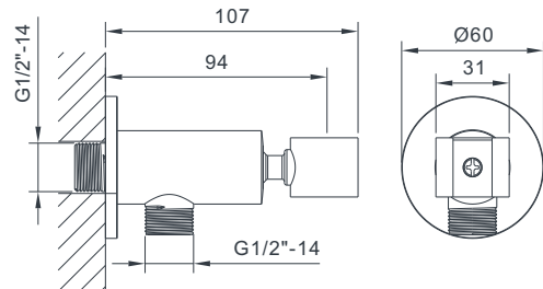
EMPORIA-04080 Built-In handshower
