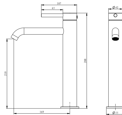
EMPORIA-03011 Basin mixer
