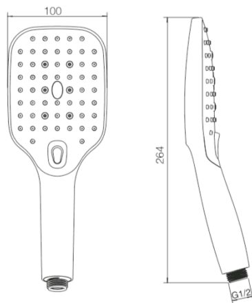
EMPORIA-040732 Shower hand
