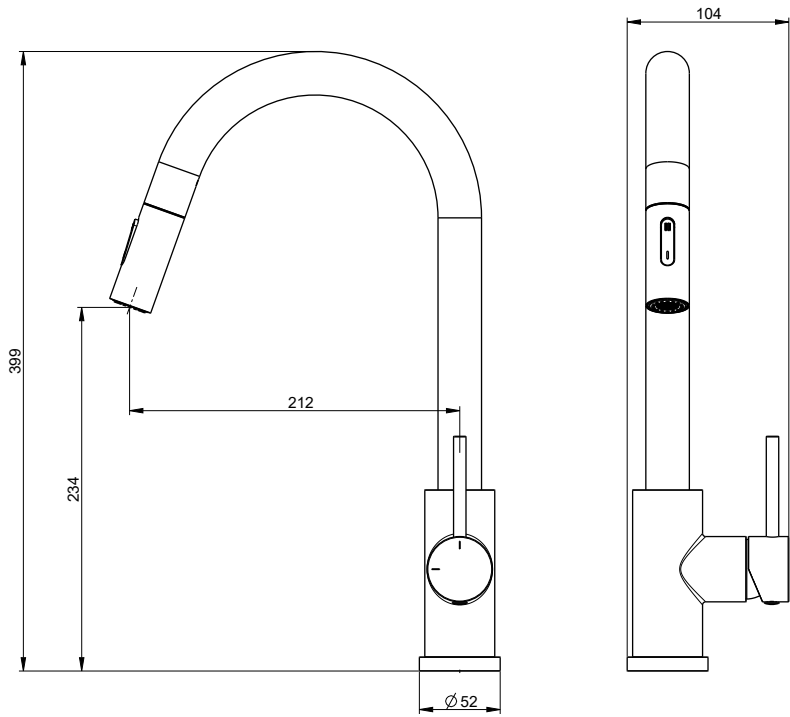
EMPORIA-060170 FAVO Kitchen faucet
