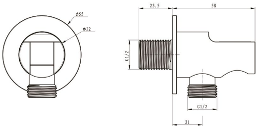
EMPORIA-04082 Built-In handshower
