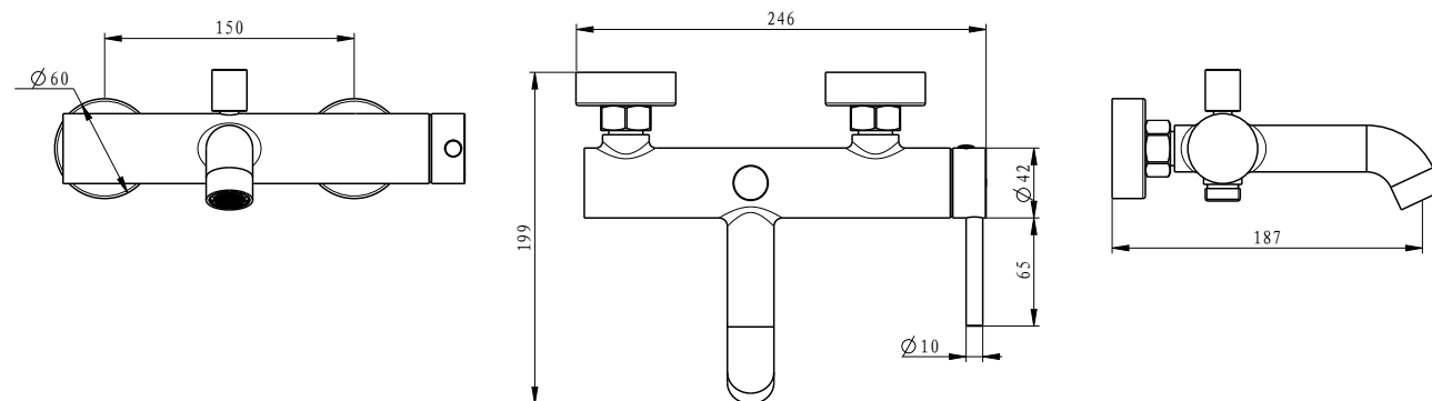
MPORIA-03030 Bath mixer
