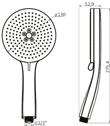
EMPORIA-040733 Shower hand
