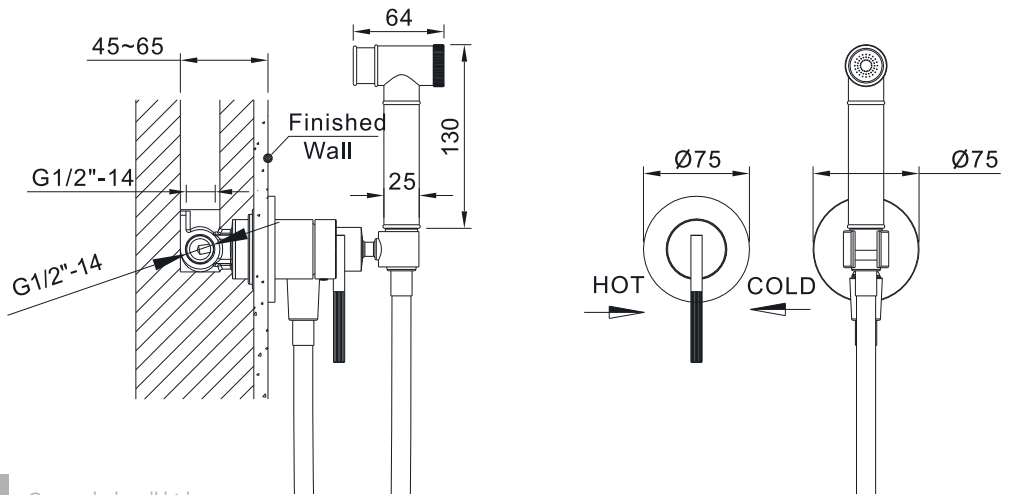
EMPORIA-01021 Concealed wall bidet
