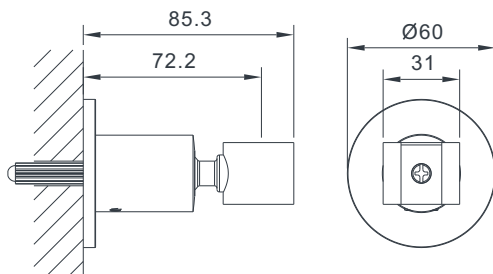
EMPORIA-04090 Shower holder
