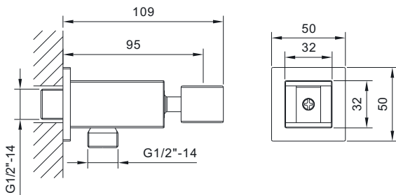
EMPORIA-04081 Built-In handshower
