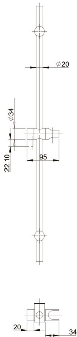
EMPORIA-040180 Shower rail adjustable
