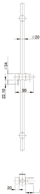
EMPORIA-040180 Shower rail adjustable
