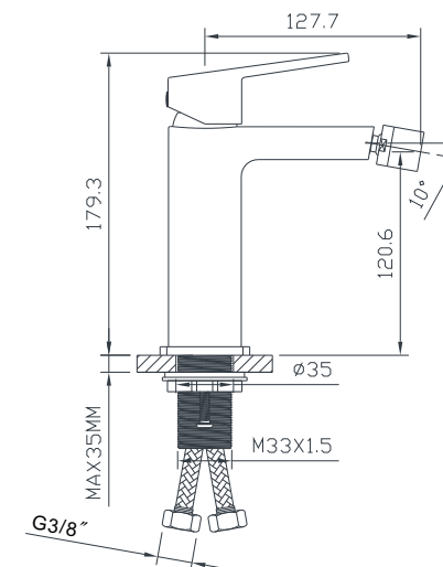
EMPORIA-02020 Bidet mixer
