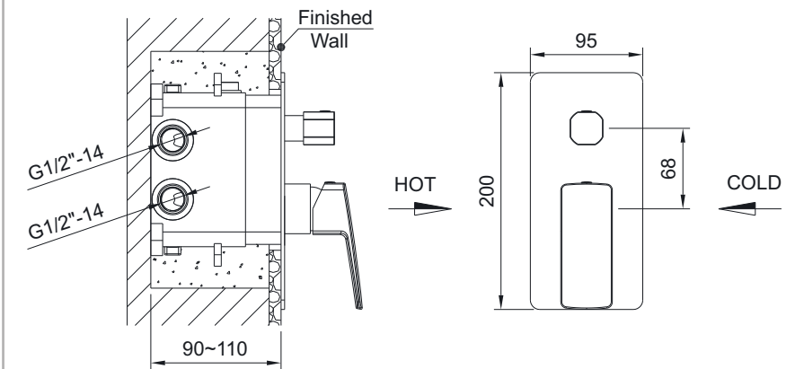
EMPORIA-02042 Concealed shower mixer
