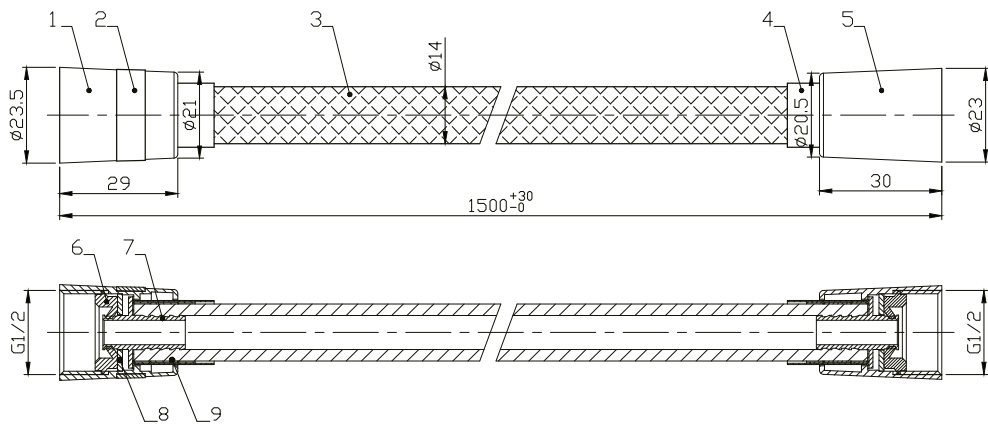
EMPORIA-0401001 Shower hose
