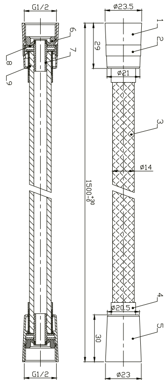
EMPORIA-040100 Shower hose
