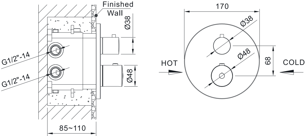
EMPORIA-01043 Concealed shower mixer
